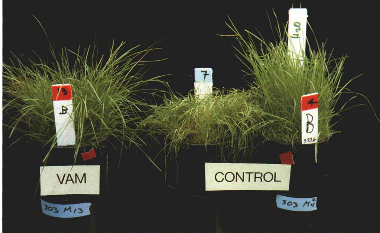
The pots at left and center were not watered for four days in the greenhouse study of drought tolerance in mycorrhizal and non-mycorrhizal creeping bentgrass. The pot on right (control) was watered daily. Note the severe wilting in the non-mycorrhizal plants (center pot) in comparison to the mycorrhizal plants (left pot).
