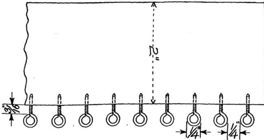
Putting green rake devised by Mr. Stewart Gardner, Chicago. A useful implement to use on the greens for raking in top-dressings. The tines are screw-eyes with one-fourth-inch eyes and set one-fourth inch apart. The lower figure is a front view of the head of the rake, full size.
