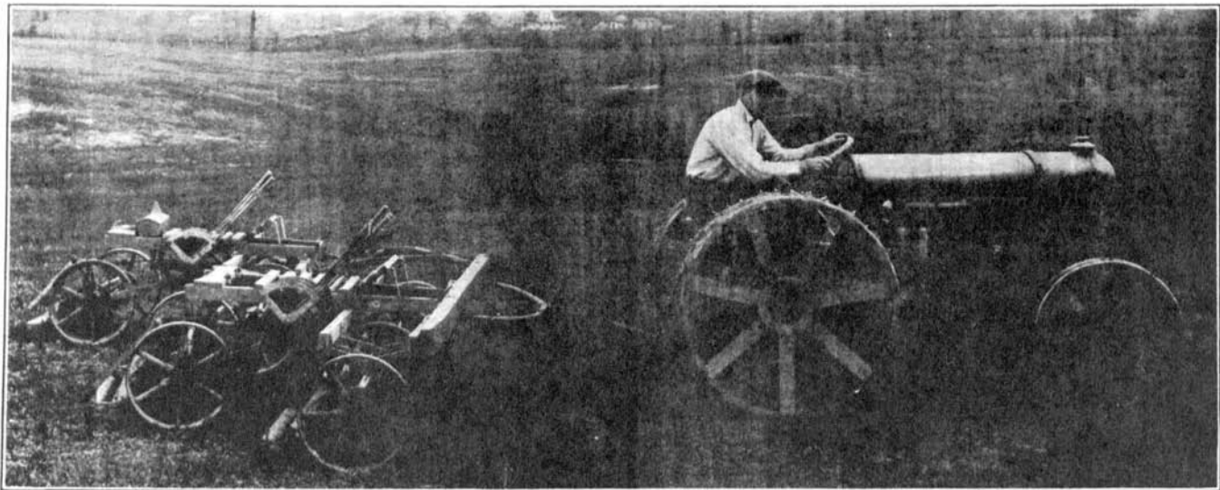
Tractor and mower combination used by the Ashtabula Country Club, Ashtabula, Ohio. Mr. Amos F. Hubbard, Secretary of the club, writes, "A bar of wood is attached by bolts to one triplex mower, extending four feet beyond this machine, for the attachment to the trailing triplex. The triplex mowers are attached by any old buggy poles. It gives flexibility in making turns and hitches close to the power. The system of attachment is simple and cheap."
