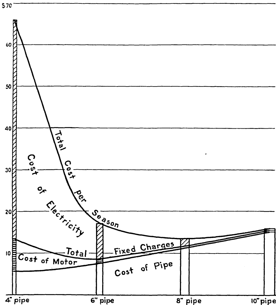
Cost of electricity is an important item in total seasonal cost in the operation of a water system. Installation of 4-inch pipe, in the particular case for which this chart was prepared, was estimated to involve a total seasonal cost of nearly $70, while 10-inch pipe would represent a total seasonal cost of a little over $15 for each 100 feet of pipe. The use of 8-inch pipe appeared from the figures obtained to be the most economical
